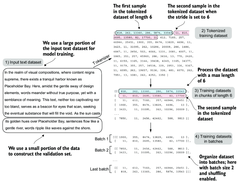
Figure 5.9 When preparing the data loaders, we split the input text into training and validation set portions. Then we tokenize the text (only shown for the training set portion for simplicity) and divide the tokenized text into chunks of a user-specified length (here, 6). Finally, we shuffle the rows and organize the chunked text into batches (here, batch size 2), which we can use for model training.
