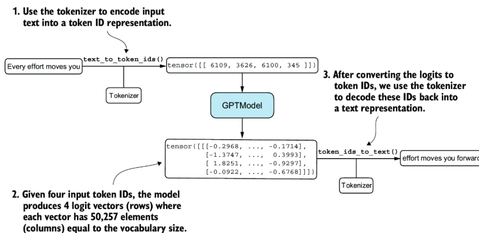
Figure 5.3 Generating text involves encoding text into token IDs that the LLM processes into logit vectors. The logit vectors are then converted back into token IDs, detokenized into a text representation.
